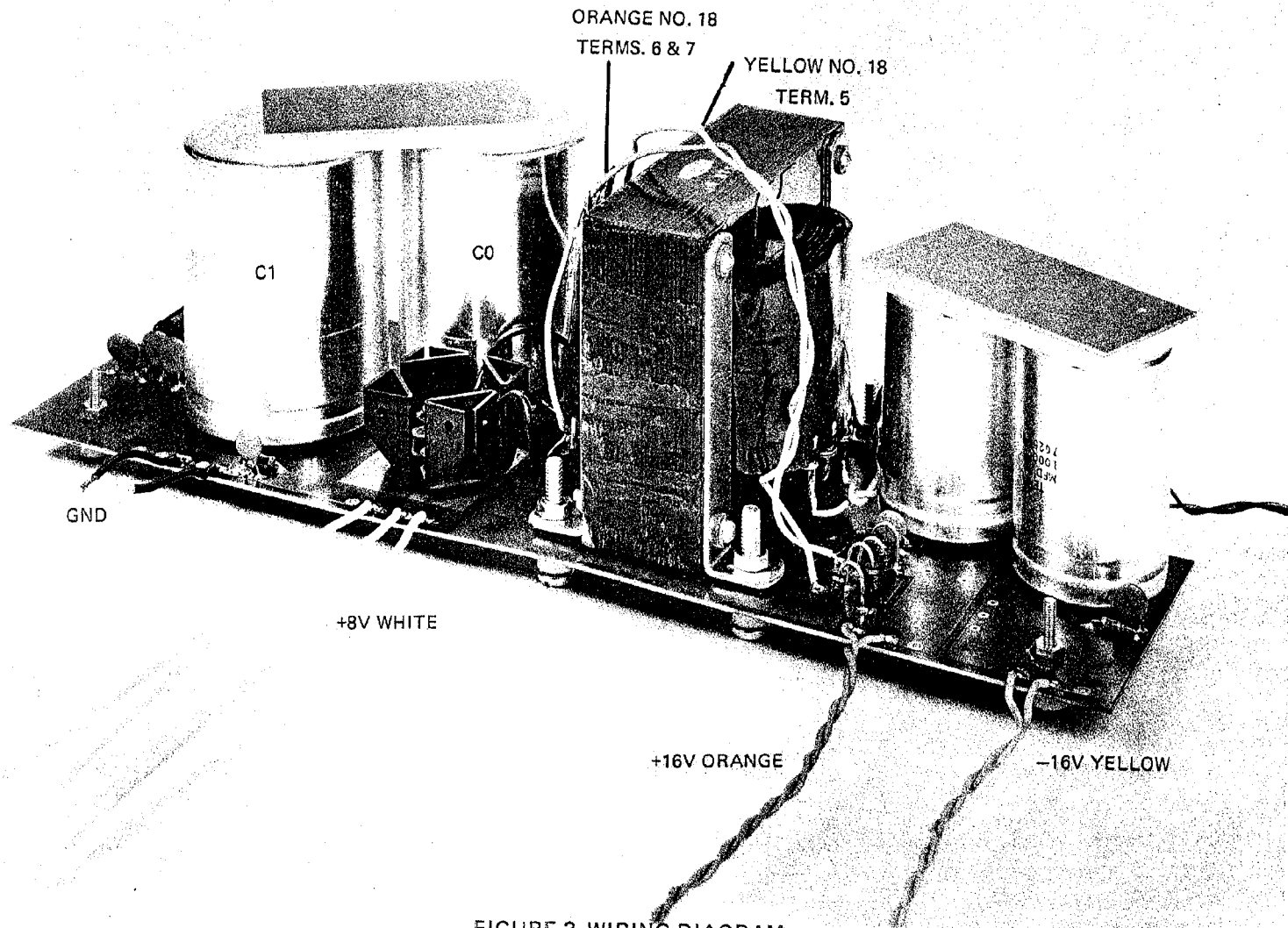
FIGURE 3 WIRING DIAGRAM
