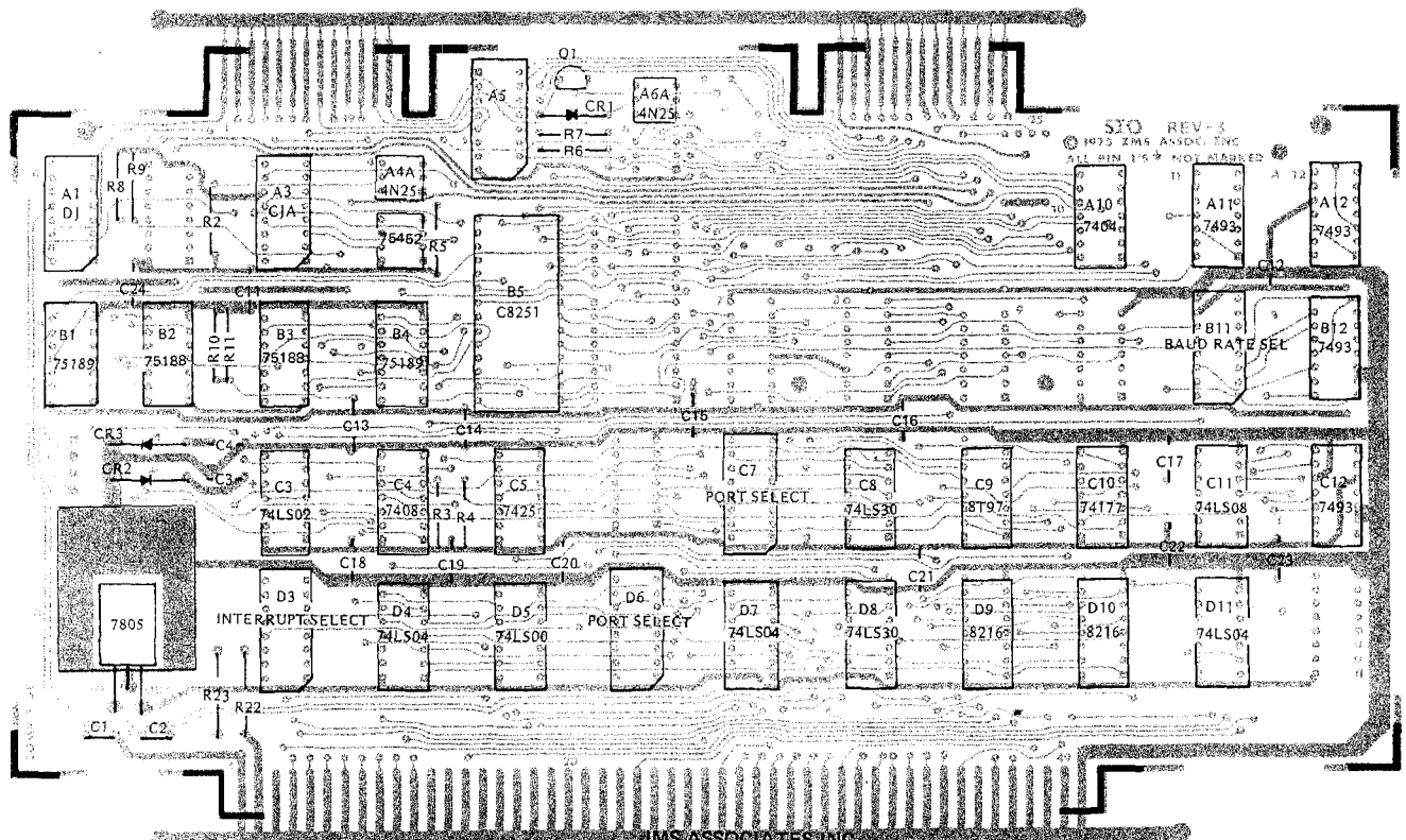
ZMS ASSOCIATES INC. ASSEMBLY DIAGRAM SIO 2-1 REV 3 2/76
