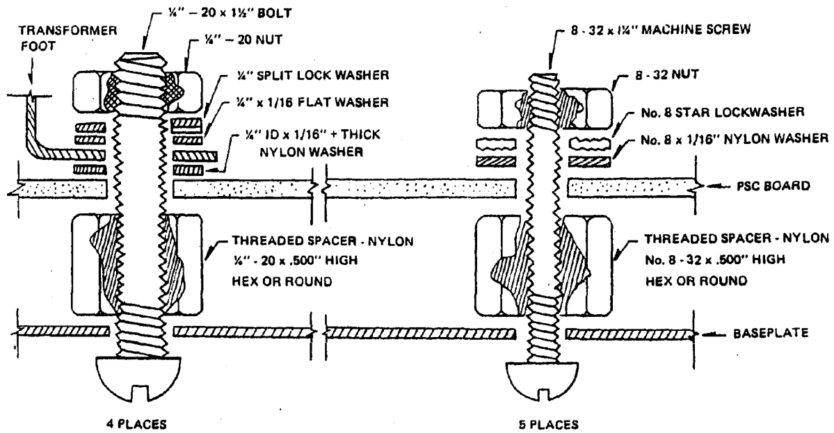
PS-C BOARD MOUNTING SYSTEMS
