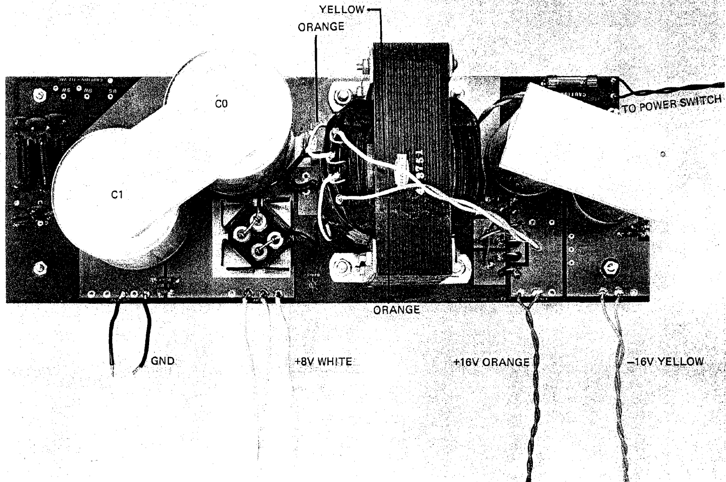
FIGURE 1 PS-28D OVERALL
