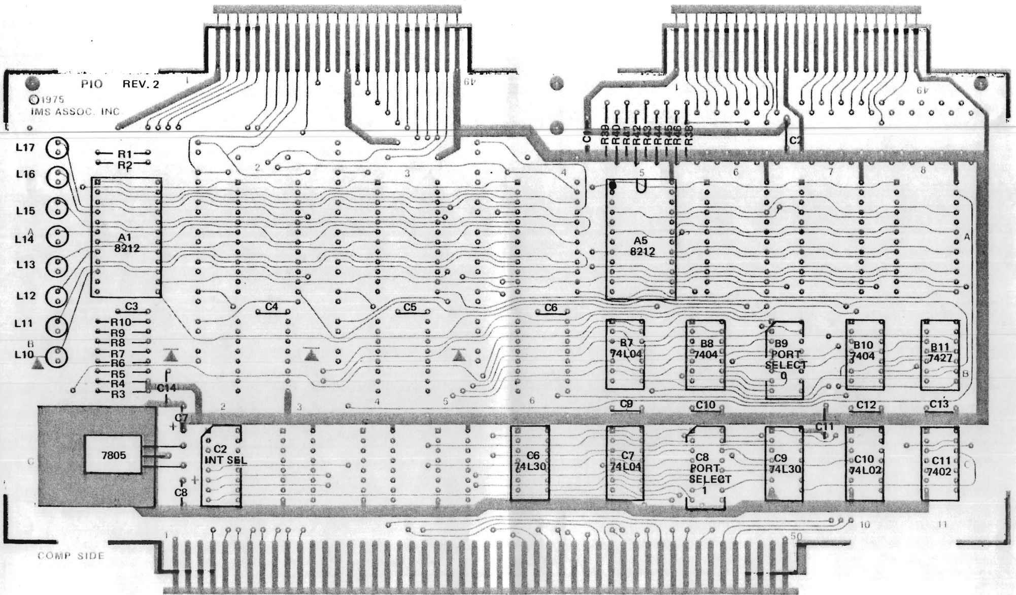
IMS ASSOCIATES INC. ASSEMBLY DIAGRAM PIO 4-1 REV. 2 5/76
