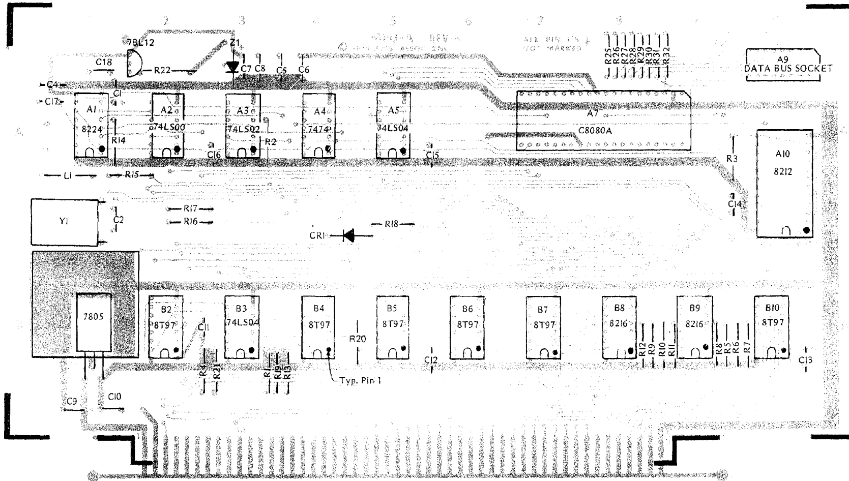
IMS ASSOCIATES INC. ASSEMBLY DIAGRAM MPU-A REV 4 2/76
